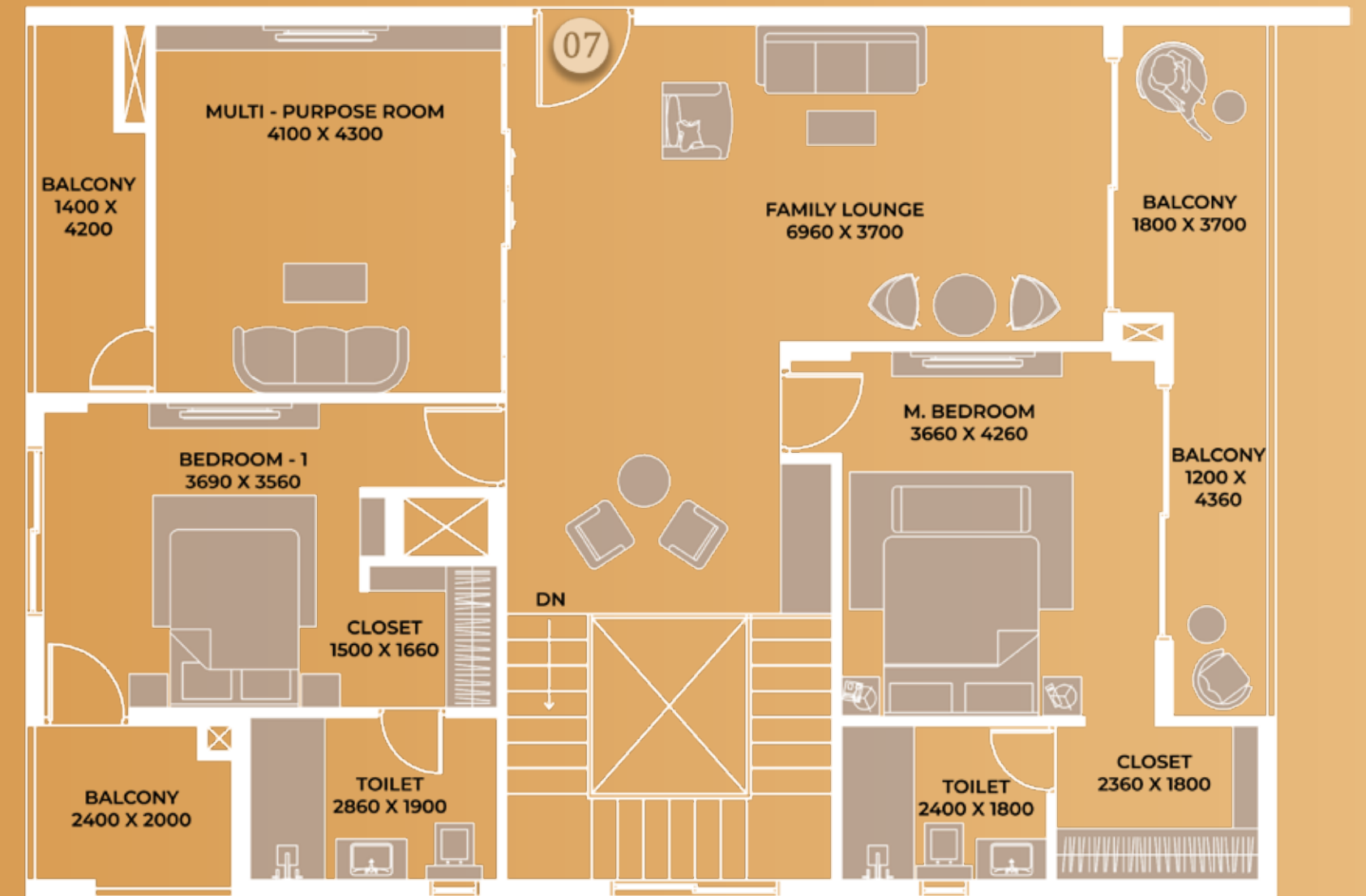
UPPER DUPLEX: 10TH FLOOR
