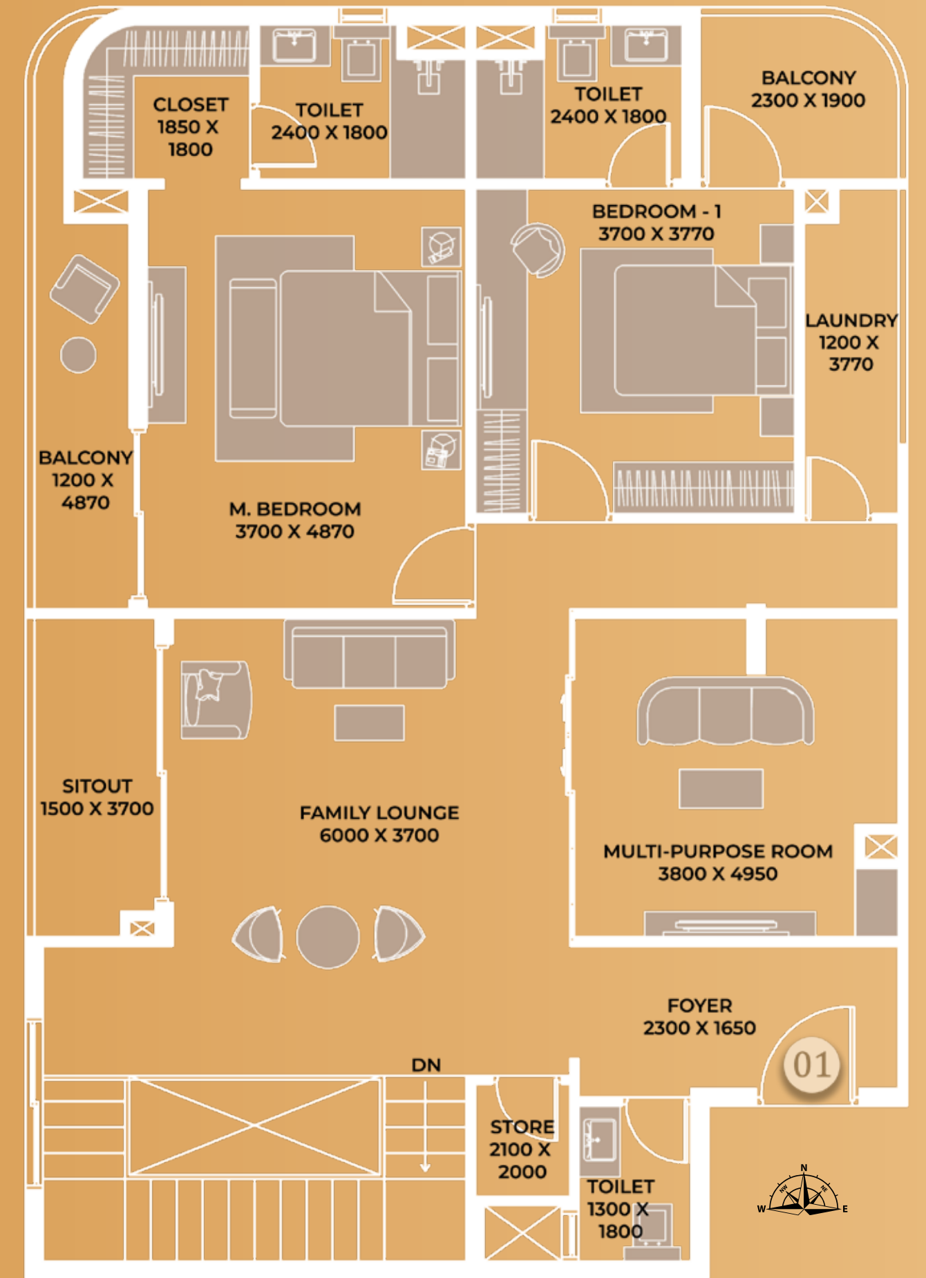
UPPER DUPLEX: 10TH FLOOR
