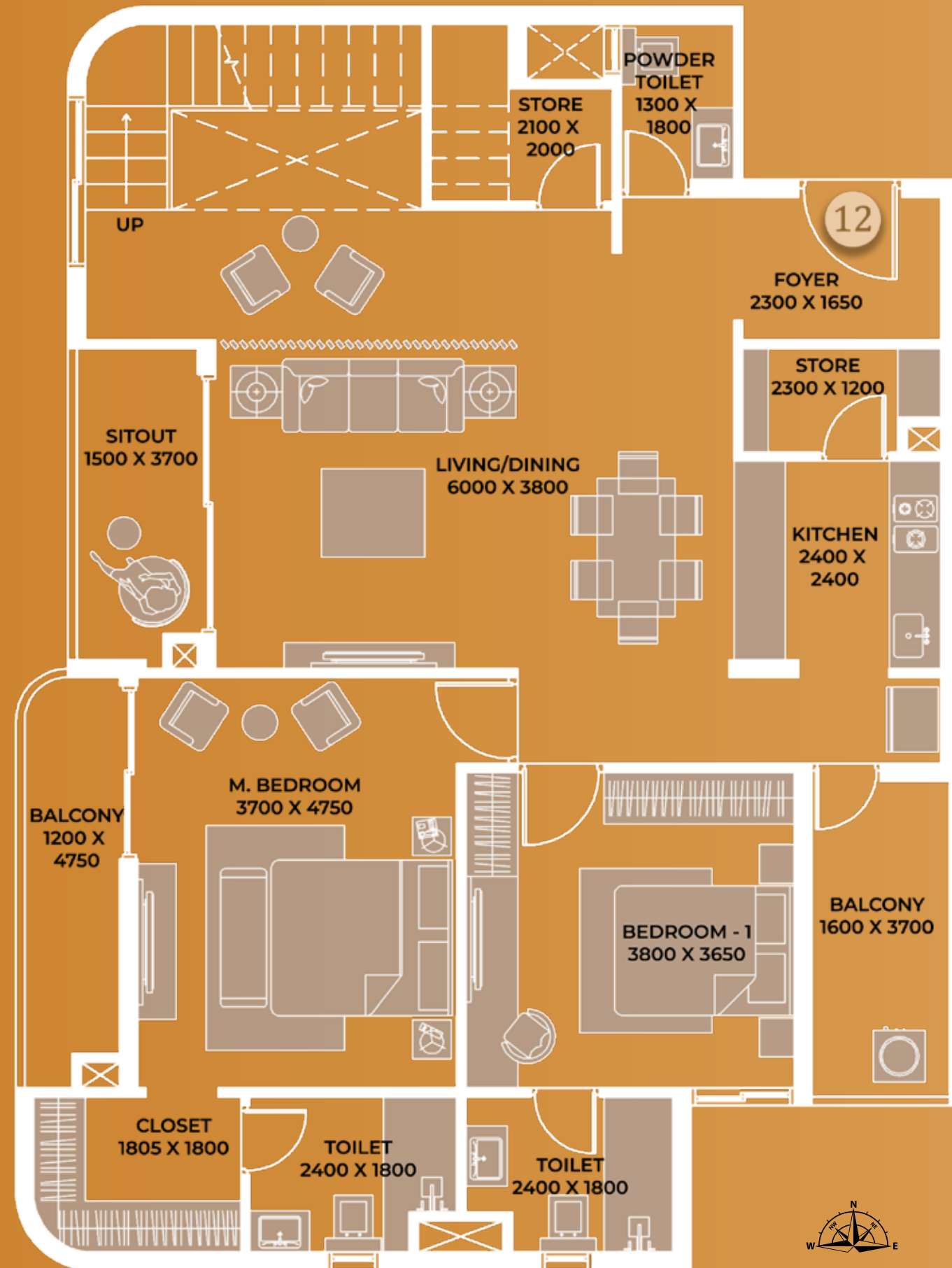
LOWER DUPLEX: 9TH FLOOR
