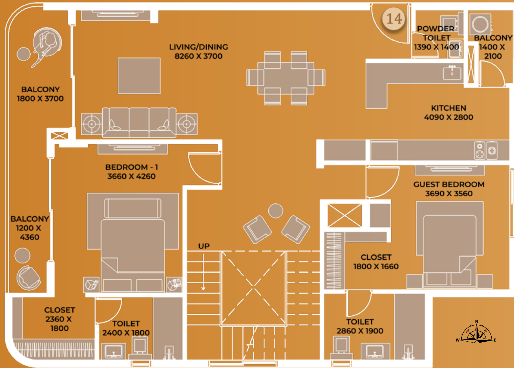
LOWER DUPLEX: 9TH FLOOR
