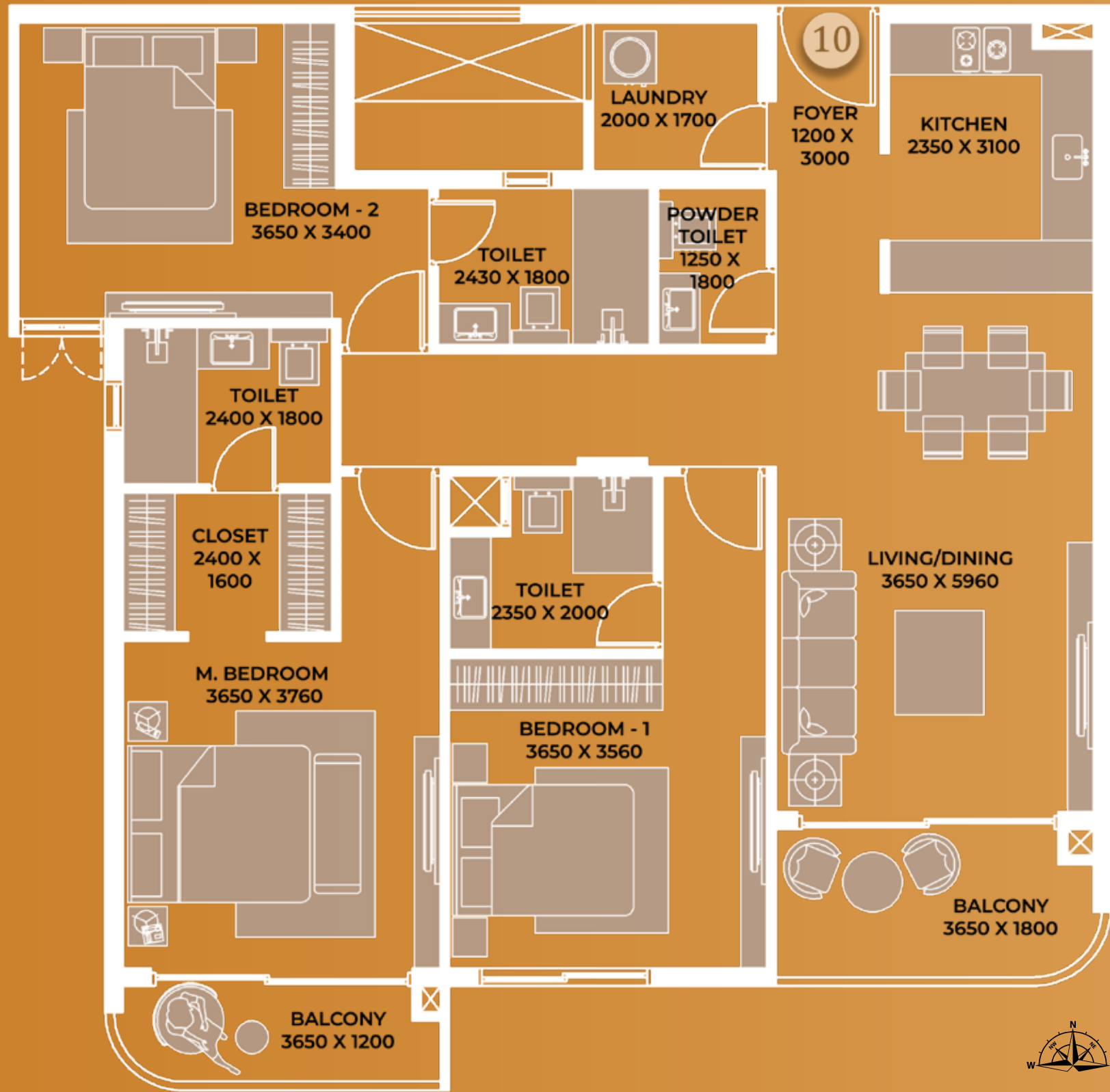
UNIT - 10 _ 3BHK (170 SQMT.) TYPICAL FLOOR
