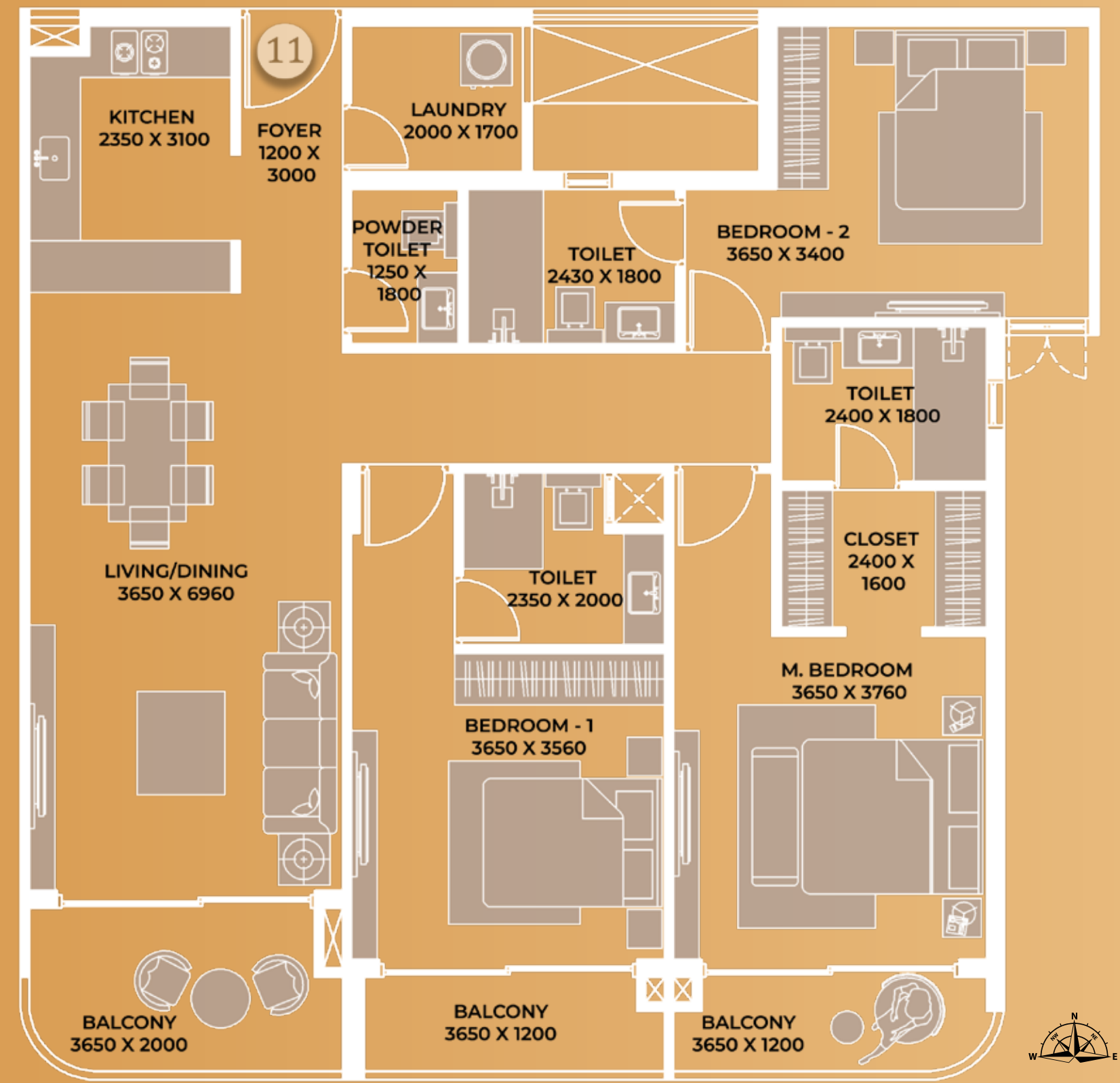
UNIT - 11 _ 3BHK (181 SQMT.) TYPICAL FLOOR
